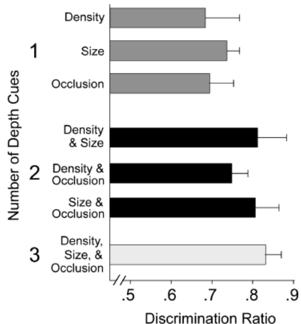
Fig. 3. Mean discrimination ratio for the 3 successful pigeons as a function of the specific depth cues present in the display during the seven steady-state probe sessions in Phase 1. Error bars show standard errors of the means.
